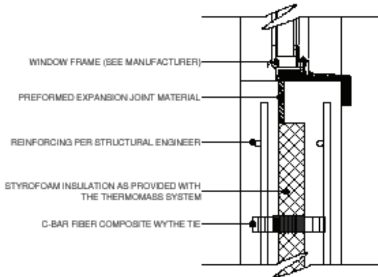
SILL DETAIL
