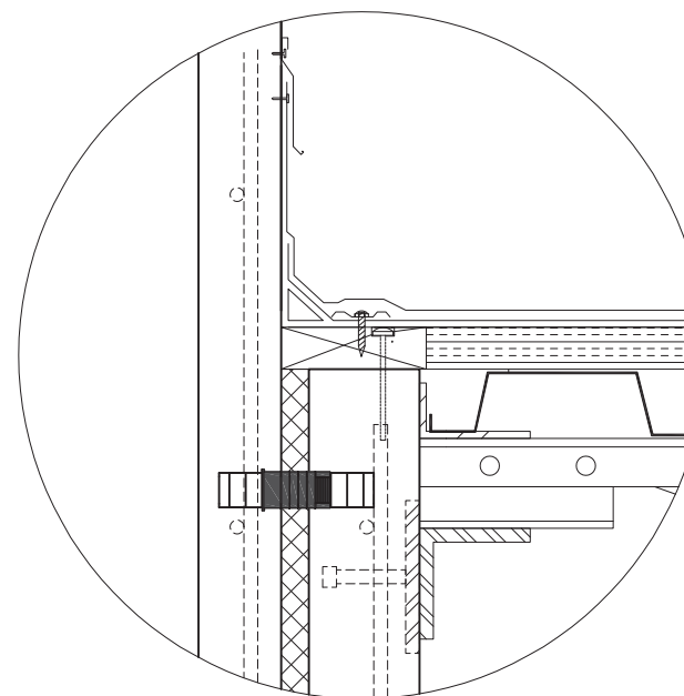
OPTIONAL CONNECTION
