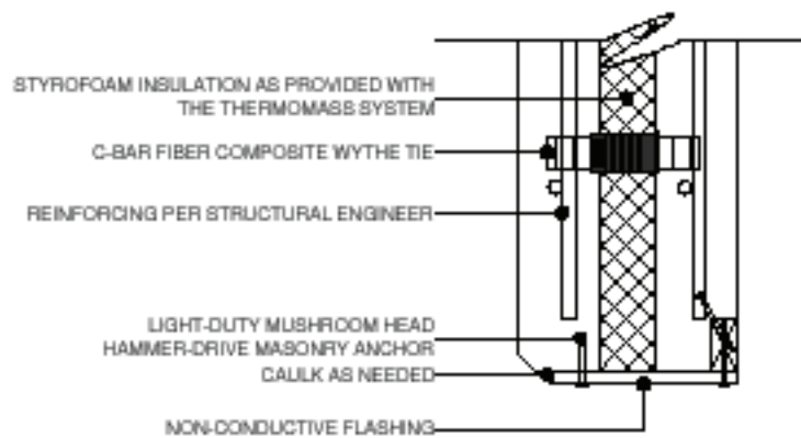
HEAD DETAIL - JAMB SIMILAR
