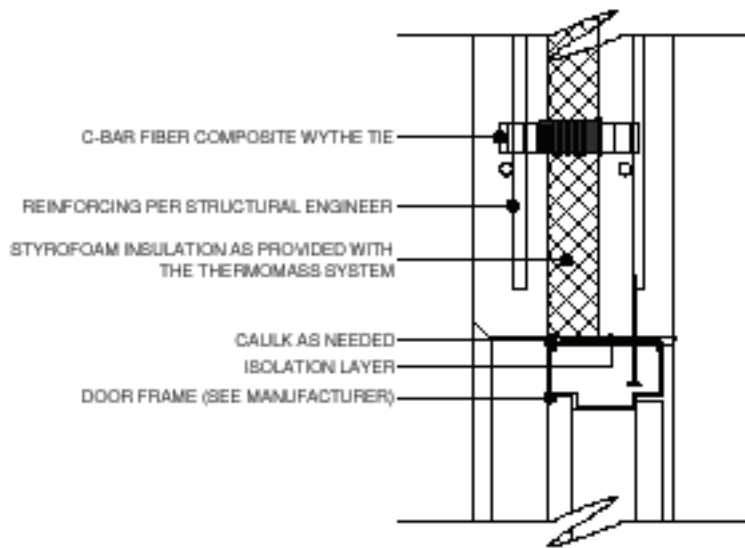
HEAD DETAIL - JAMB SIMILAR
